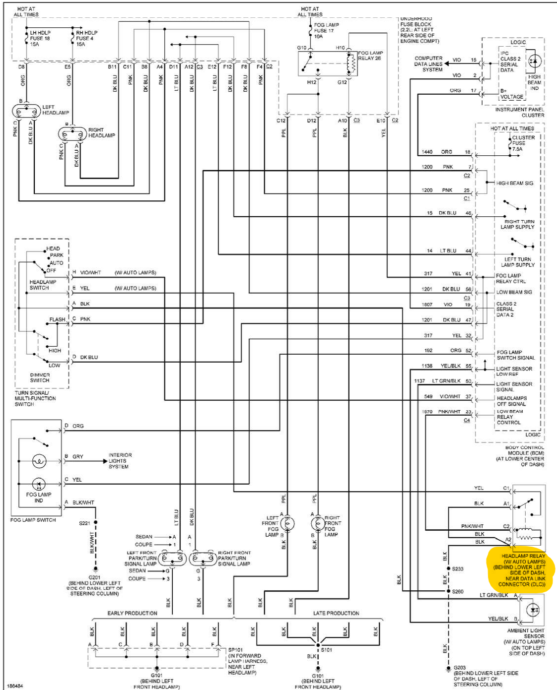
Fig. 24: Headlamps & Fog Lamps Circuit
